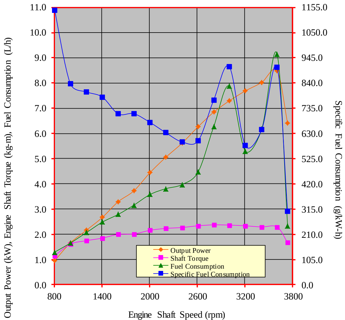
Figure 3. Performance characteristic curves of the BLUMAX BXD 195F diesel engine
