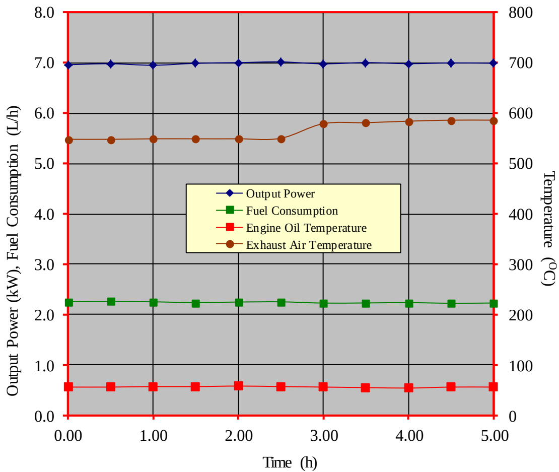
Figure 4. Performance characteristic curves during the continuous running test BLUMAX BXD 195F diesel engine
